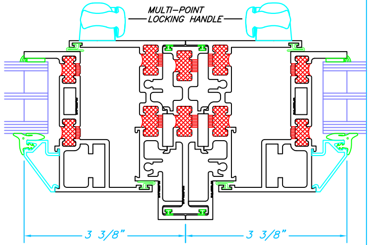
11 VERTICAL MULLION Ⓞ PROJECT OUT OR CASEMENT / PROJECT OUT OR CASEMENT VENT
